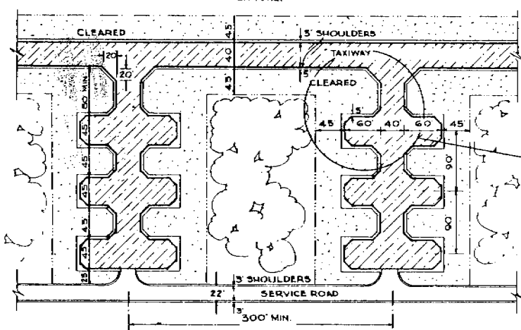
FIG. 1 HARDSTAND DETAILS
