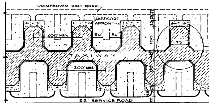
HARDSTAND DETAIL
